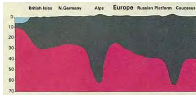
Figure 2: Schematic section. The mountains, like pegs, have deep roots embedded in the ground. 2750
